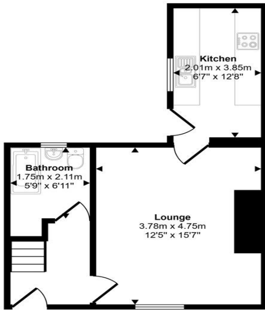
Ground Floor Approx 35 sq m / 382 sq ft
