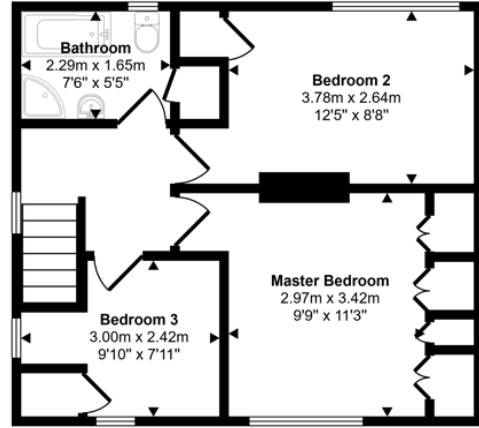
First Floor Approx 43 sq m / 468 sq ft
