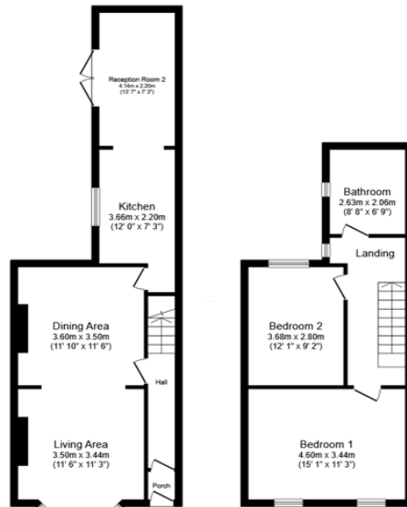
Ground Floor Floor area 51.8 sq.m. (558 sq.ft.)
